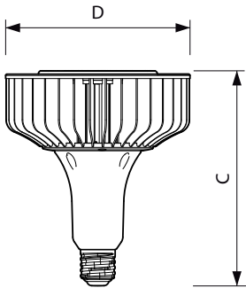
TrueForce Core HB 200-160W E40 840 NB LA
