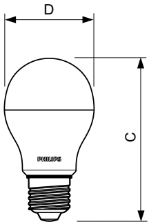
Bulb A55 11-95W 1250lm 6500K E27
