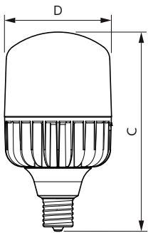
TForce HB 70-65W E40 865 200D
