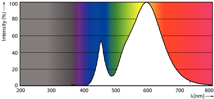
Spectral Power Distribution Colour - EcoHome LEDBulb 4W E27 3000K G45 1PF AR
