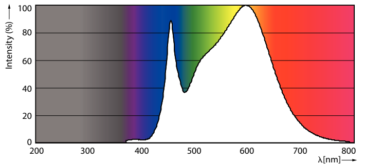
LED PAR30L 28W 840 100-277V
