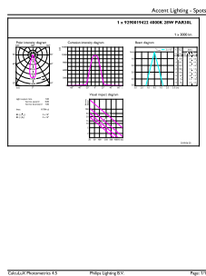
LED PAR30L 28W 30D 840 100-277V
