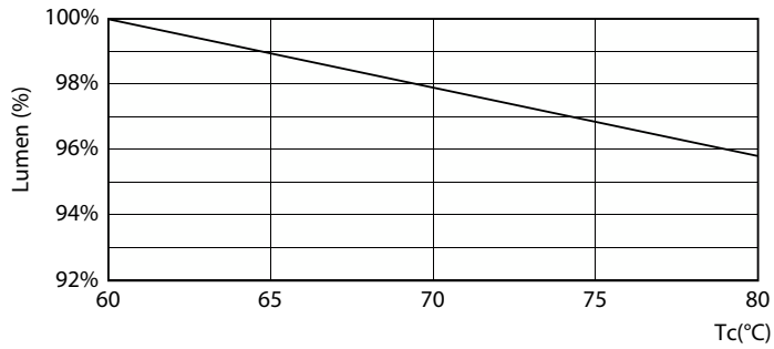
LEDtube MAS LATAM 8W 50K LumenVsTc-LMP
