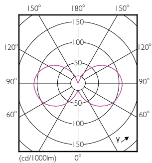
LEDcapsule_1,6W_G9
