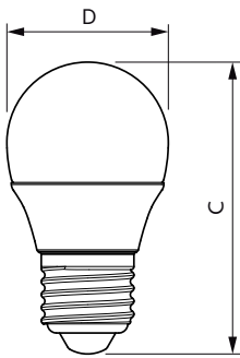
Bulb 230V 3.5-32W 350lm 3000K E27 ND
